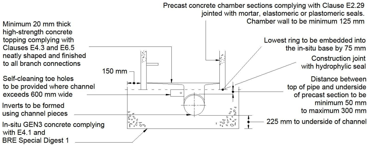
Figure B10: Alternative base detail for Type A and Type B manholes without concrete surround
